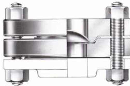
Figure 29: Bolted type fitting with flat faced flanges.
