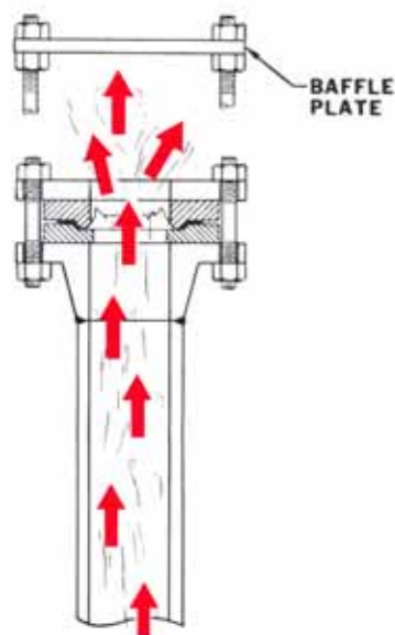
Figure 9: Rupture disk installed so overpressure impulse is transmitted directly to disk.
